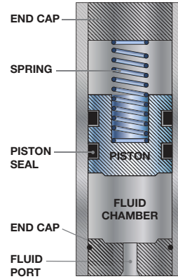
SPRING TYPE
