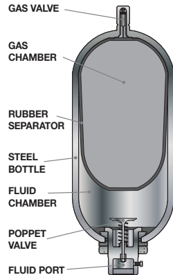
BLADDER TYPE
