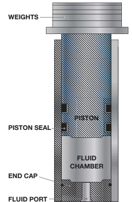
WEIGHT LOADED
