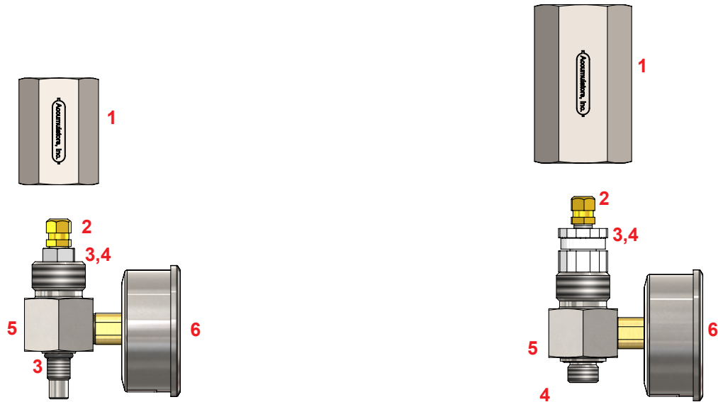
3000 PSI
