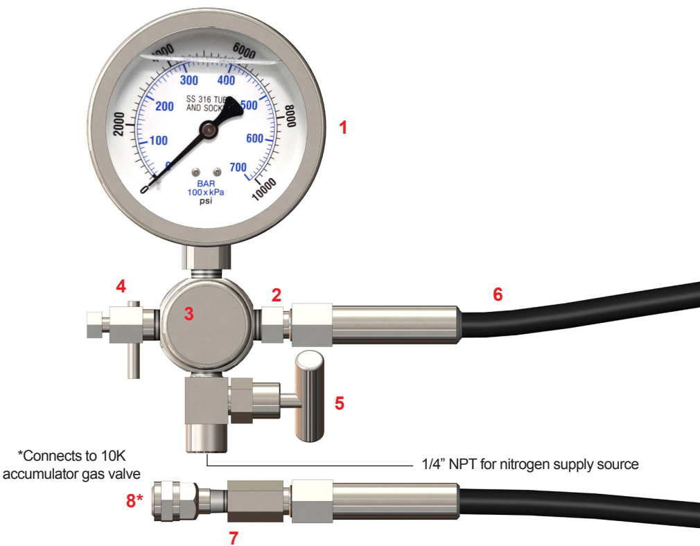
10000 PSI CHARGING AND GAUGING ASSEMBLY
