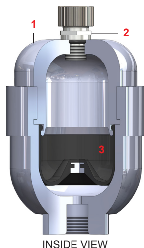
INSIDE VIEW
